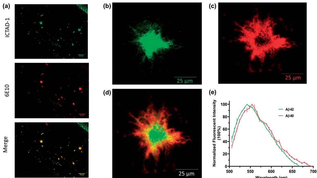
Fig. 5 (a) The brain tissues from 5xFAD mice were co-stained with ICTAD-1 and antibody 6E10; (b) the core of A \beta plaque stained with ICTAD-1; (c) the periphery of A \beta plaque stained with ICTAD-1; (d) merged image of (b) and (c); (e) the normalized unmixing fluorescent spectra of A \beta plaques stained with ICTAD-1 ( n = 3 ).
