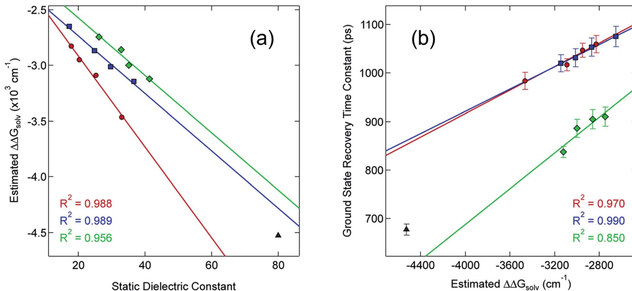
Fig. 5 Correlating the estimated change in \Delta G_{\text{solv}} ( \Delta\Delta G_{\text{solv}} , eqn (4)) between the HS and LS states of [\text{Fe}(\text{bpy})_3]^{2+} with (a) the static dielectric constant and (b) the time constants for ground state recovery in alcohol-based (red circles), nitrile-based (blue squares), and diol-based (green diamonds) solutions. The result for water (black triangle) is listed in both, but is not included in any of the linear fits.
