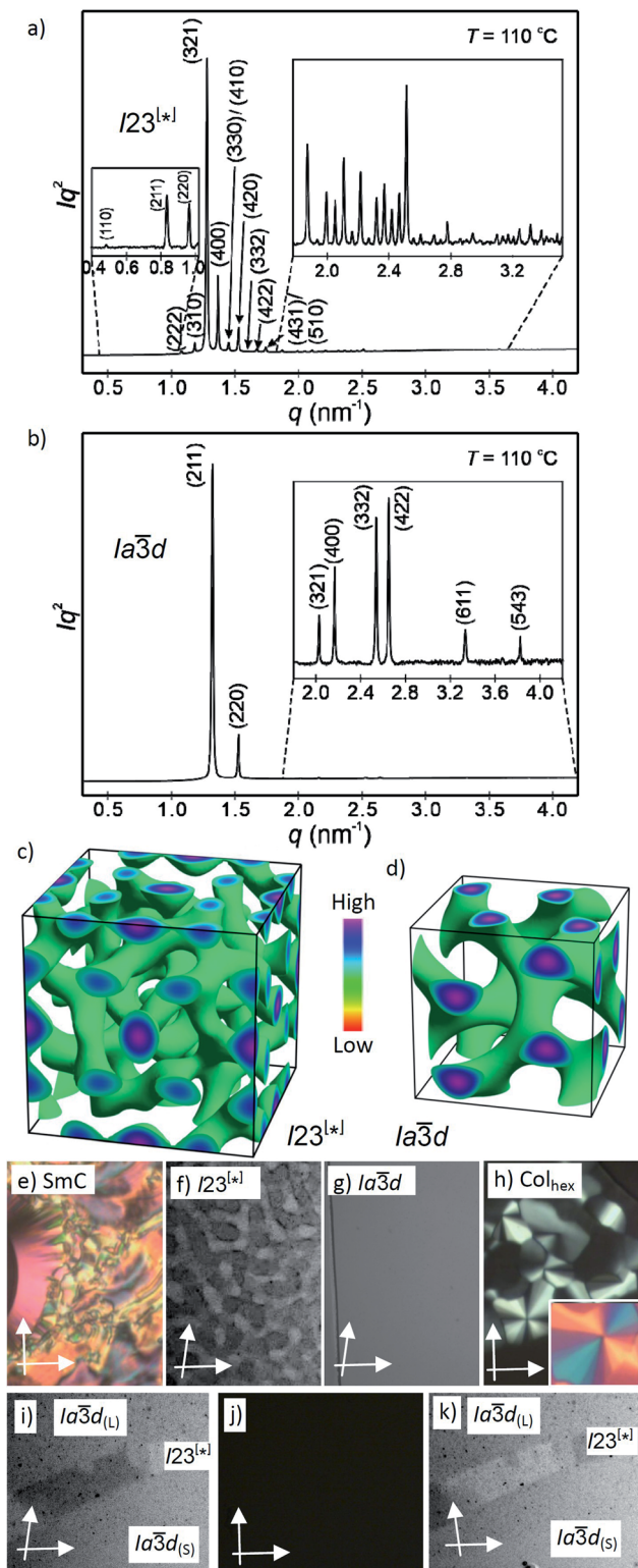
Fig. 2 (a and b) SAXS diffractograms of the I23^{[*]} (3/4) and the Ia\bar{3}d (3/16) phases (for the synchrotron source and for numerical data, see Tables S4 and S5;† the full indexations of the I23^{[*]} phase and the WAXS scans are shown in Fig. S7†); (c and d) reconstructed electron density maps of the I23^{[*]} and Ia\bar{3}d phases; the aromatic cores are located in the networks formed by the green iso-surfaces, the space between is filled by the alkyl chains; for more details, see the ESI, and Fig. S8† for the individual networks; (e–h) the textures of the (e) SmC phase of 3/10 at 230^\circ\text{C} ; (f) the \text{Cub}_{\text{bi}}/I23^{[*]} phase of 3/10 at 121^\circ\text{C} and
