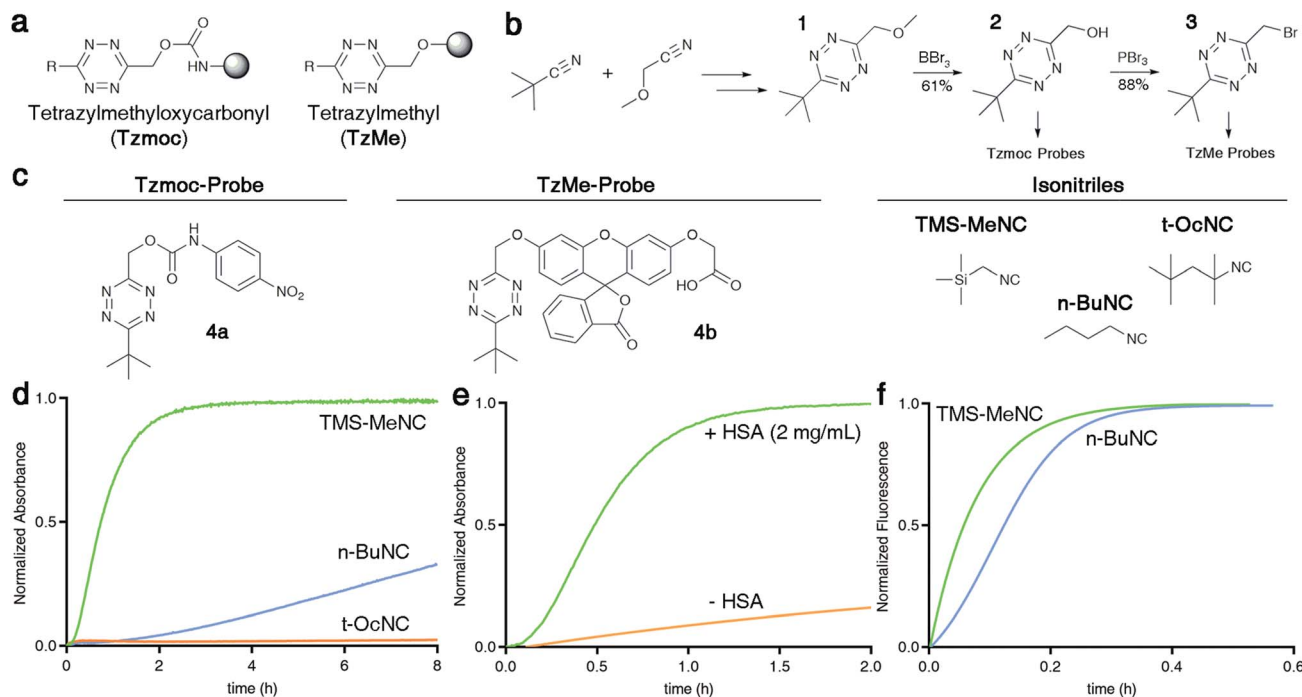
Fig. 2 Isonitrile-mediated uncaging of amines and phenols from Tzmc and TzMe derivatives. (a) Structures of tetrazylmethoxycarbonyl (Tzmc) and tetrazylmethyl (TzMe) groups used to cage amines and phenols, respectively. (b) Synthesis of Tzmc or TzMe-caged probes (conditions and yields described in the ESI†). (c) Structures of reporter probes and isonitrile triggers used in this study. (d) Kinetics of pNA release from 4a triggered by different isonitriles (c(4a) = 0.2 mM, c(R-NC) = 2 mM, DMSO : PBS pH 7.4 (4 : 1, v/v), T = 37 °C, λ = 435 nm, n = 3). (e) Kinetics of pNA release from 4a triggered by n-BuNC catalysed by serum albumin (c(4a) = 8 μM, c(n-BuNC) = 6 mM, c(HSA) = 2 mg mL -1 , DMSO : PBS pH 7.4 (1 : 4, v/v), T = 37 °C, λ = 385 nm, n = 3). (f) Kinetics of O-carboxymethyl fluorescein release from 4b triggered by TMS-MeNC or n-BuNC (c(4b) = 8 μM, c(R-NC) = 6 mM, DMSO : PBS pH 7.4 (1 : 4, v/v), T = 37 °C, λ ex = 488 nm, λ em = 520 nm, n = 3).
