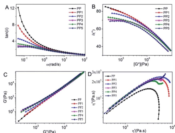
Fig. 3 \tan(\delta) – \omega relationship of (A), relation between \delta – G^* (B), Han's curves ( G' – G'' , C) and Cole–Cole curves ( \eta' – \eta'' , D) of polypropylene-based composites.
