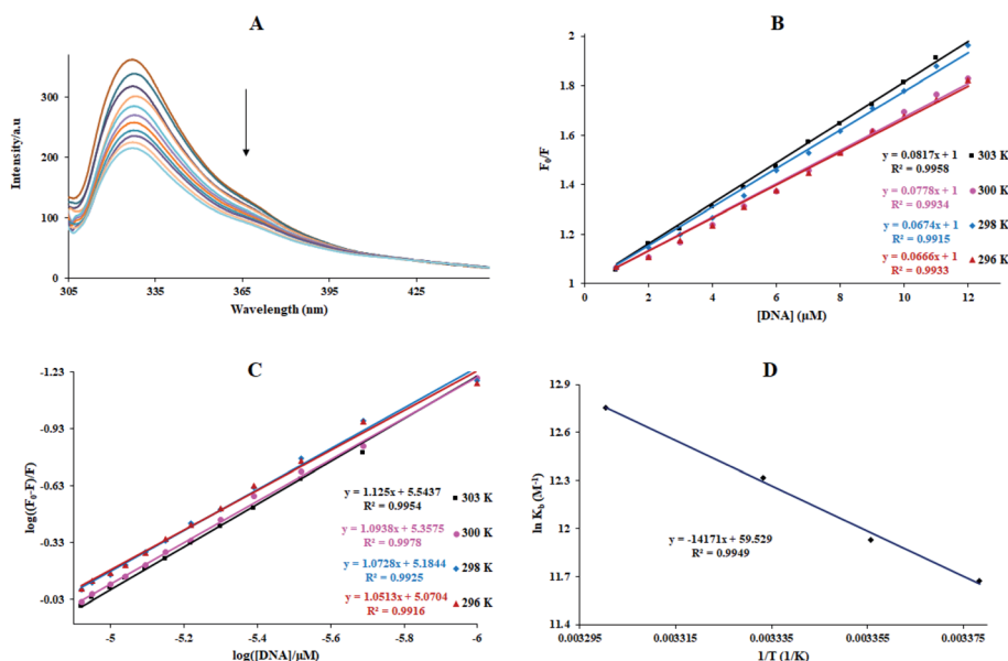
Fig. 3 (A) The fluorescence spectra of the Sm(III) complex in the presence and absence of different concentrations of DNA, [DNA] = 0 to 14.3 μM and [Complex] = 1 \times 10^{-7} M ( \lambda_{\text{ex}} = 280 nm, pH = 7.2 and T = 298 K). (B) Stern–Volmer curves, (C) Plots of \log((F_0 - F)/F) against \log([DNA]/\mu\text{M}) for the complex at 296, 298, 300 and 303 K, (D) van't Hoff plot for the interaction of DNA with the Sm(III) complex.
