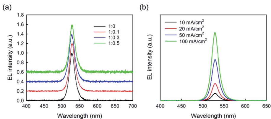
Fig. 8 (a) Normalized EL spectra of the PeLEDs with PEDOT:PSS HTLs doped with different GO amount tested at the current density of 50 mA cm -2 . (b) EL spectra for the PeLED with the optimal PEDOT:PSS:GO (1 : 0.3) HTL tested by using different current densities.
