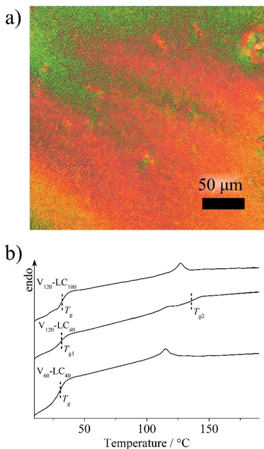
Fig. 5 (a) The POM image of the composite based on \text{pVP}_{120} - b - \text{pPhM}_{100} and (b) DSC curves of the composites based on the LC diblock copolymers.
