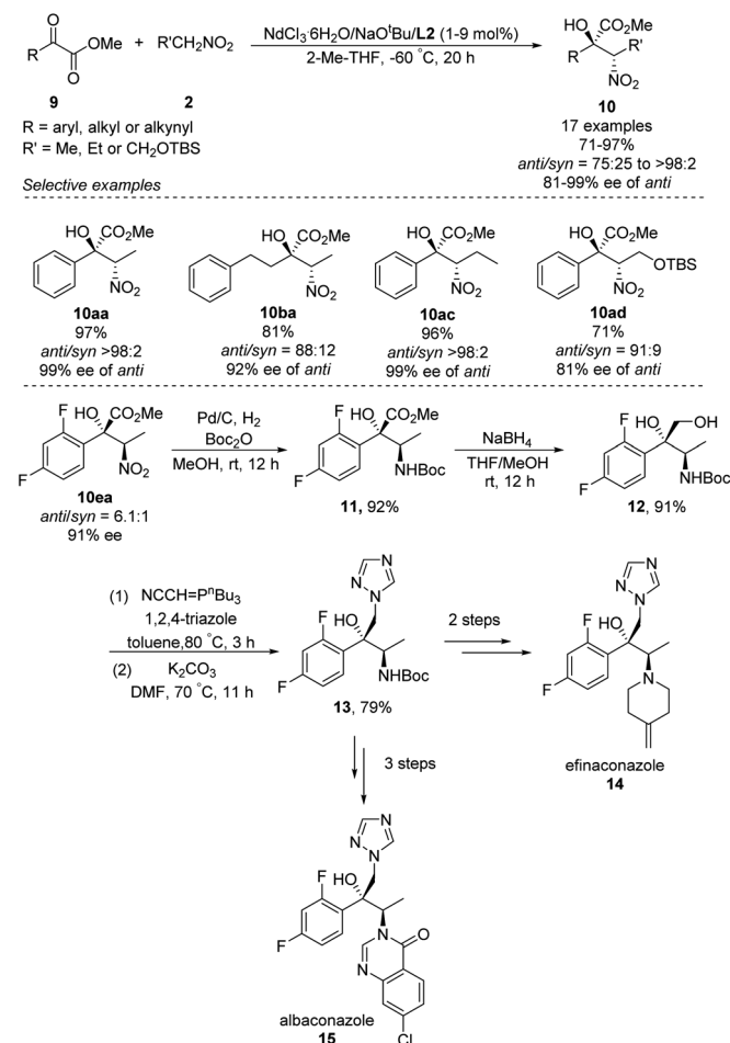
Scheme 9 Anti -selective asymmetric Henry reaction of \alpha -keto esters.
