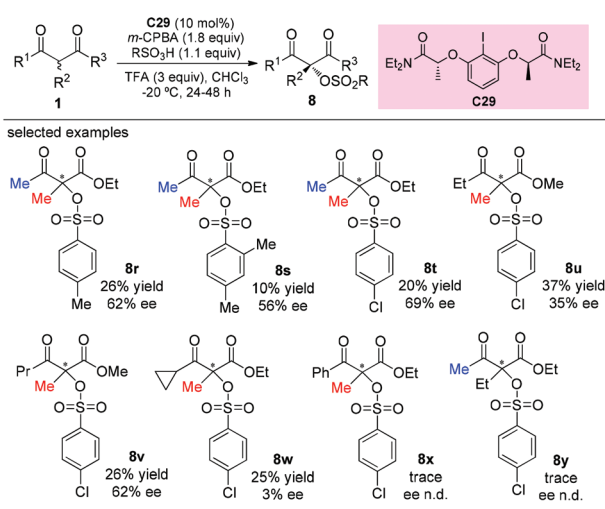
Scheme 52 Asymmetric oxidation of \alpha -substituted \beta -ketoesters promoted by C_2 -symmetric iodoarene.
