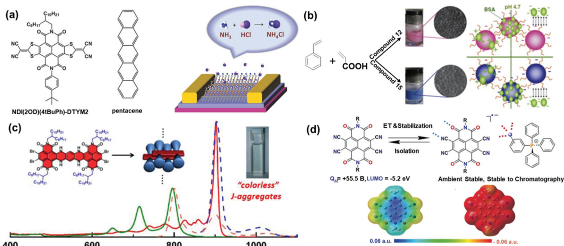
Fig. 4 (a) Molecular structures of the n-type TBNDI derivative and p-type pentacene, and a schematic diagram of the device structure and sensing mechanism. Reproduced with permission. 113 Copyright 2014, Wiley-VCH. (b) Preparation of self-colored nanoparticles containing TBNDI derivatives. Reproduced with permission. 20 Copyright 2011, Elsevier. (c) Schematic representation of the proposed packing motifs of the studied bis-TBNDIs and absorption (solid) and emission (dash) spectra ( 1.0 \times 10^{-6} M) in CHCl 3 (green and pink) and n -hexane (red and blue). Reproduced with permission. 64 Copyright 2014, American Chemical Society. (d) Structure of compound 140 and its radical anion compound 139 stabilized by supramolecular interactions. ESP (electrostatic surface potential) maps of compound 140 (left) and its radical anion (right). ESP contours are color-coded from red (electron-rich) to blue (electron-deficient). Reproduced with permission. 78 Copyright 2018, Wiley-VCH.
