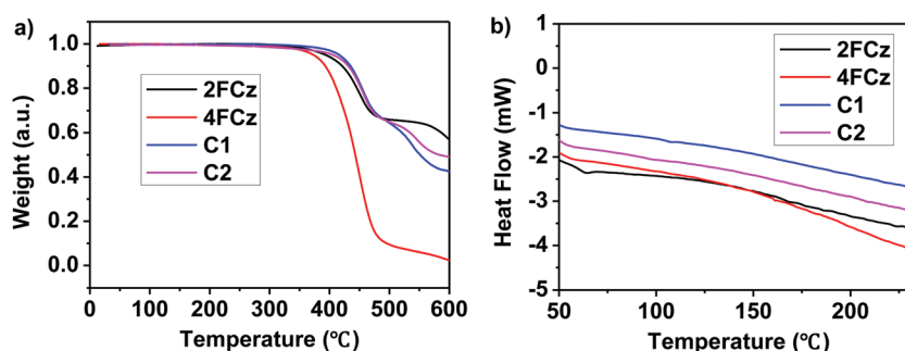
Fig. 1 (a) TGA thermograms and (b) DSC curves of xFCz and Cx at a heating rate of 10 °C min -1 .
