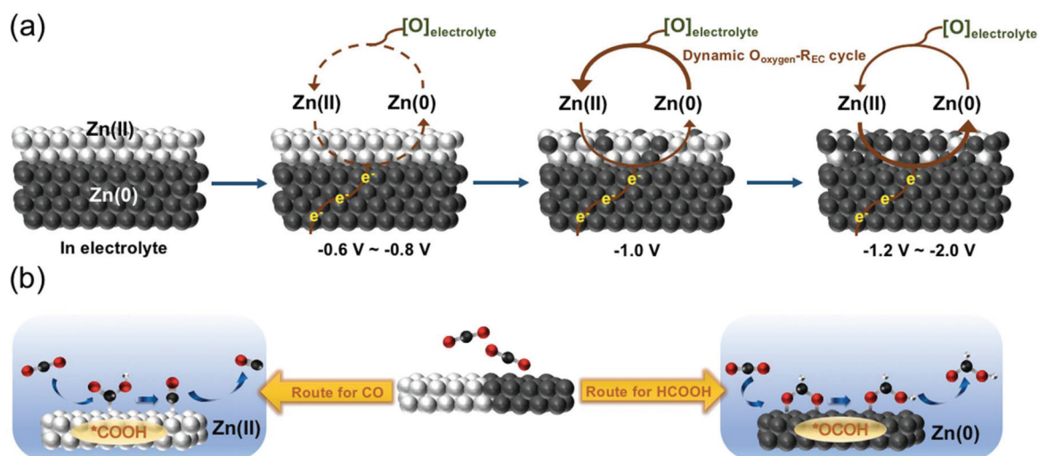
Fig. 7 (a) Schematic process of the zinc electrocatalyst during the CO 2 RR. (b) Schematic mechanisms of the CO 2 RR for Zn(II) and Zn(0) electrocatalysts.
