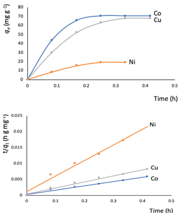
Fig. 7 Top: Metal adsorption capacity (mg g -1 ) versus time (h) plot. The solid lines is a guide to the eye; bottom: simulation of the experimental data to the pseudo-second order kinetic model. The solid lines represent the fitting of the data.
