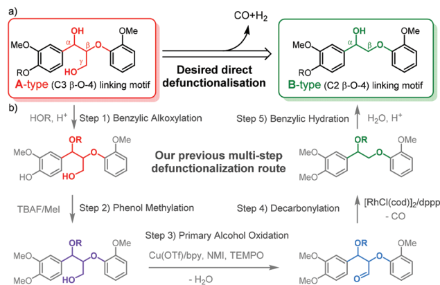
Fig. 1 (a) The two types of β-O-4 linkage motifs commonly represented in model compounds used in the chemical methodology development for lignin valorisation and (b) multistep defunctionalisation of alcohol incorporated organosolv lignin via methylation, oxidation and decarbonylation demonstrated in our previous work. 31
