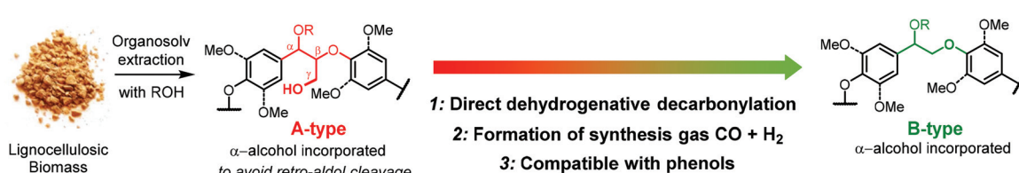
Fig. 2 (a) Overview of the primary alcohol dehydrogenation and hydrogen shuttling for in situ stabilisation of depolymerisation products of lignin developed by Bruijninx et al. 30 (b) Dehydrogenative decarbonylation of a series of simple primary alcohols demonstrated by Madsen et al. 40 (c) Direct dehydrogenative decarbonylation to defunctionalize a high alcohol incorporated lignin demonstrated in this work.
