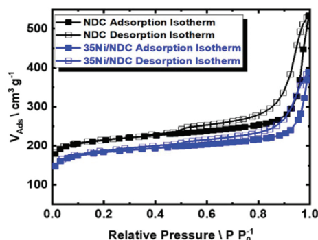
Fig. 4 N_2 sorption isotherm at 77 K of the parent NDC and 35Ni/NDC.
