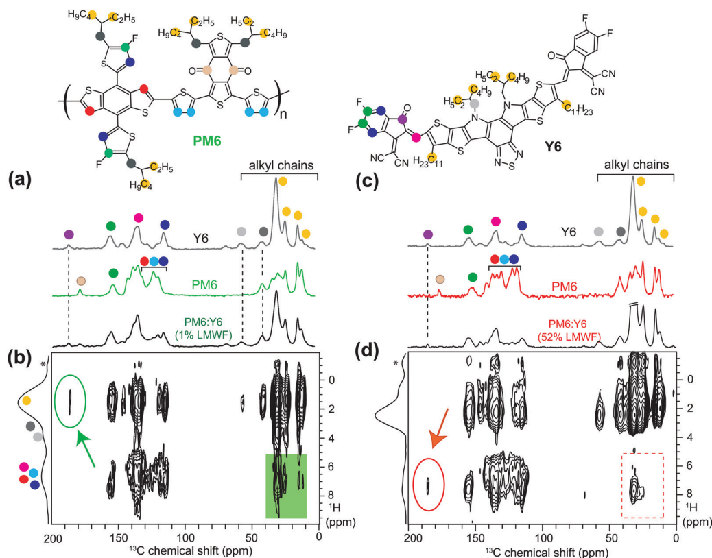
Fig. 4 Left: Comparison of (a) 1D ^{13}\text{C}\{^1\text{H}\} CP-MAS spectra of neat Y6, PM6 (1% LMWF) and PM6:Y6 blends. (b) 2D ^{13}\text{C} - ^1\text{H} heteronuclear correlation NMR spectrum of 1% LMWF PM6:Y6 blend. Right: Comparison of (c) 1D ^{13}\text{C}\{^1\text{H}\} CP-MAS spectra of neat Y6, PM6 (52% LMWF), and PM6:Y6 blends. (d) 2D ^{13}\text{C} - ^1\text{H} heteronuclear correlation NMR spectrum of 52% LMWF PM6:Y6 blend. Spectra were acquired at 9.4 T (12.5 kHz MAS) with 4 ms of CP contact time. * denotes the carrier frequency of ^1\text{H} homonuclear decoupling.
