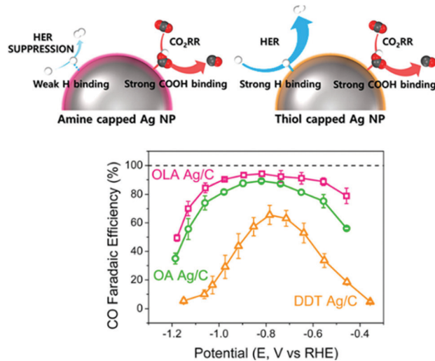
Fig. 33 Schematic illustration of amine- and thiol-capped Ag NPs for \text{CO}_2 RR. CO faradaic efficiency as a function of the applied potential for oleylamine (OLA)-capped Ag/C, oleic acid (OA)-capped Ag/C, and dodecanethiol (DDT)-capped Ag/C. Reproduced with permission from ref. 424. Copyright 2017 American Chemical Society.
