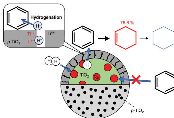
Fig. 4 Selective hydrogenation of benzene over (Ru/TiO 2 )@p-TiO 2 .
