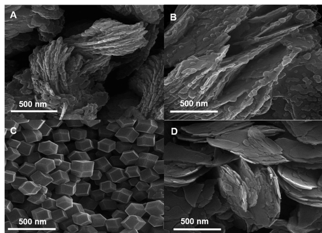
Fig. 2 FESEM images of the synthesized ZIF-8 with linker/metal molar ratios of A) 4.0, B) 10.0, and C) 20.0 in the presence of GA and D) 20.0 in the absence of GA at a total volume of 10.0 ml.
