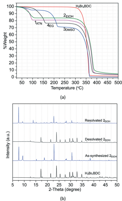
Fig. 5 TG curves of H 2 Br 4 BDC and all the solvates (a) and PXRD patterns (bottom to top) of H 2 Br 4 BDC, as synthesized 2 EtOH , desolvated 2 EtOH , and resolved 2 EtOH (b).
