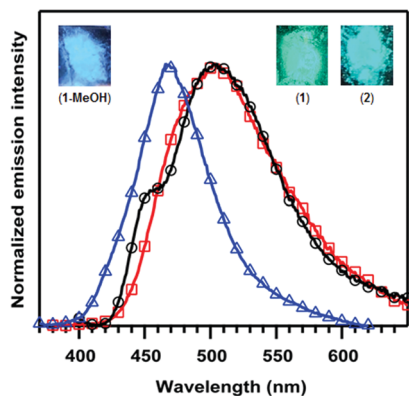
Fig. 2 Emission spectra for 1 (red; \square ), 2 (black; \circ ) and 1-MeOH (blue; \Delta ) in the solid-state. Photoluminescence colours for 1 , 2 , and 1-MeOH are provided at the upper right or left corners of the figure. Data were collected every 1 nm, and the symbols are present to help distinguish the overlaid plots.
