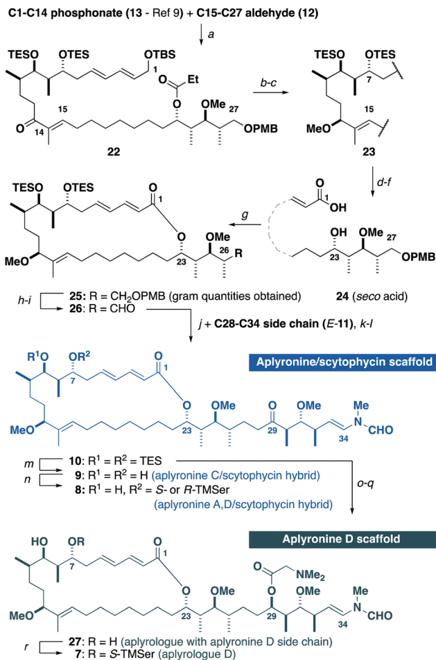
Scheme 4 Synthesis of aplyrologues. Reagents and conditions: (a) \text{Ba}(\text{OH})_2 , THF/ \text{H}_2\text{O} (40:1), r.t., 85%, >20:1 E/Z, (b) R -MeCBS, \text{BH}_3\cdot\text{SMe}_2 , -10^\circ\text{C} , 93%, >20:1 dr, (c) \text{Me}_3\text{O}\cdot\text{BF}_4 , Proton Sponge ® , \text{CH}_2\text{Cl}_2 , r.t., 87%, (d) DIBAL, \text{CH}_2\text{Cl}_2 , -78^\circ\text{C} , 99%, (e) DDQ, \text{CH}_2\text{Cl}_2/\text{pH} 9.2 buffer (4:1), 0^\circ\text{C} to r.t., 75%, 91% brsm, (f) \text{NaClO}_2 , \text{NaH}_2\text{PO}_4\cdot\text{H}_2\text{O} , 2-methyl-but-2-ene, \text{H}_2\text{O}/t\text{BuOH} , 0^\circ\text{C} to r.t., (g) TCBC, \text{Et}_3\text{N} ; DMAP, PhMe, r.t., 70% over two steps, (h) DDQ, \text{CH}_2\text{Cl}_2/\text{pH} 7.0 buffer (2:1), r.t., 82%, (i) DMP, \text{NaHCO}_3 , \text{CH}_2\text{Cl}_2 , r.t., (j) E-11 , \text{Cy}_2\text{BCl} , \text{Et}_3\text{N} , \text{Et}_2\text{O} , 0^\circ\text{C} ; 26 , \text{Et}_2\text{O} , -78 to -10^\circ\text{C} , (k) Burgess reagent, THF, r.t., 65% over three steps, (l) \text{Cu}(\text{OAc})_2 , PPh 3 , TMS, PhMe, r.t., 89%, (m) HF-py/py (1:2), THF, 0^\circ\text{C} to r.t., 85%, (n) TCBC, R - or S -TMSer, \text{Et}_3\text{N} , DMAP, PhH, 62% for S-8 , 73% for R-8 , (o) \text{Zn}(\text{BH})_4 , \text{Et}_2\text{O} , 0^\circ\text{C} , 58%, 2:1 dr, (p) DMGly, DCC, DMAP, DMAP-HCl, r.t., (q) HF-py/py (1:2), THF, 0^\circ\text{C} to r.t., 69% over two steps, (r) TCBC, S -TMSer, \text{Et}_3\text{N} , DMAP, PhH, 65%. CBS: Corey–Bakshi–Shibata catalyst.
