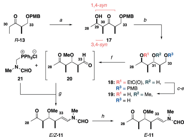
Scheme 3 Synthesis of the C28–C34 ketone E-11 . Reagents and conditions: (a) R-13 , \text{Ti}(\text{O}i\text{Pr})\text{Cl}_3 , DIPEA, \text{CH}_2\text{Cl}_2 , -78^\circ\text{C} ; acetaldehyde, \text{CH}_2\text{Cl}_2 , -78^\circ\text{C} , 77%, 17 : 1 dr, (b) \text{SmI}_2 , EtCHO, THF, -20^\circ\text{C} , 97%, >20:1 dr, (c) \text{Me}_3\text{O}\cdot\text{BF}_4 , Proton Sponge ® , \text{CH}_2\text{Cl}_2 , r.t., 90%, (d) DDQ, \text{CH}_2\text{Cl}_2/\text{pH} 7 buffer (2:1), r.t., 93%, (e) DIBAL, \text{CH}_2\text{Cl}_2 , -78^\circ\text{C} , 87%, (f) (\text{COCl})_2 , DMSO, \text{CH}_2\text{Cl}_2 , -78^\circ\text{C} ; \text{Et}_3\text{N} , -78^\circ\text{C} to r.t., (g) 21 , LiHMDS, THF, -78^\circ\text{C} ; 20 , THF -78 to -20^\circ\text{C} , 60% over two steps, 3:1 Z/E, (h) \text{I}_2 (5 mol%), \text{CH}_2\text{Cl}_2 , r.t., 86%, >20:1 E/Z.
