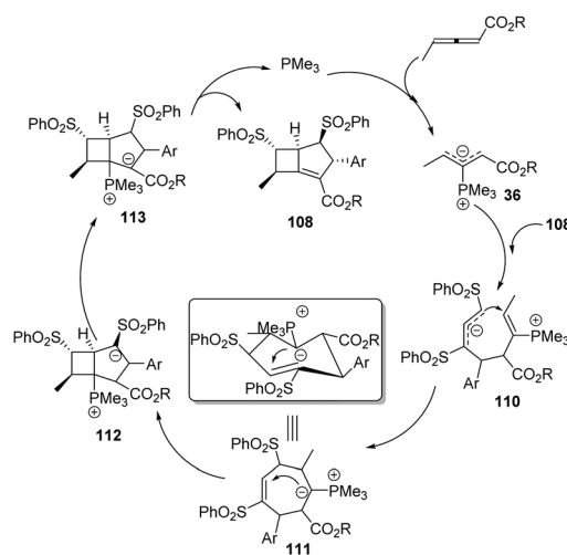
Scheme 35 The proposed mechanism for the synthesis of bicyclo[3.2.0]heptene derivatives.
