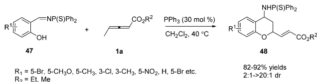
Scheme 14 Phosphine-catalysed abnormal (2+4) annulations of \gamma -methyl allenates with N -thiophosphinylamines.
