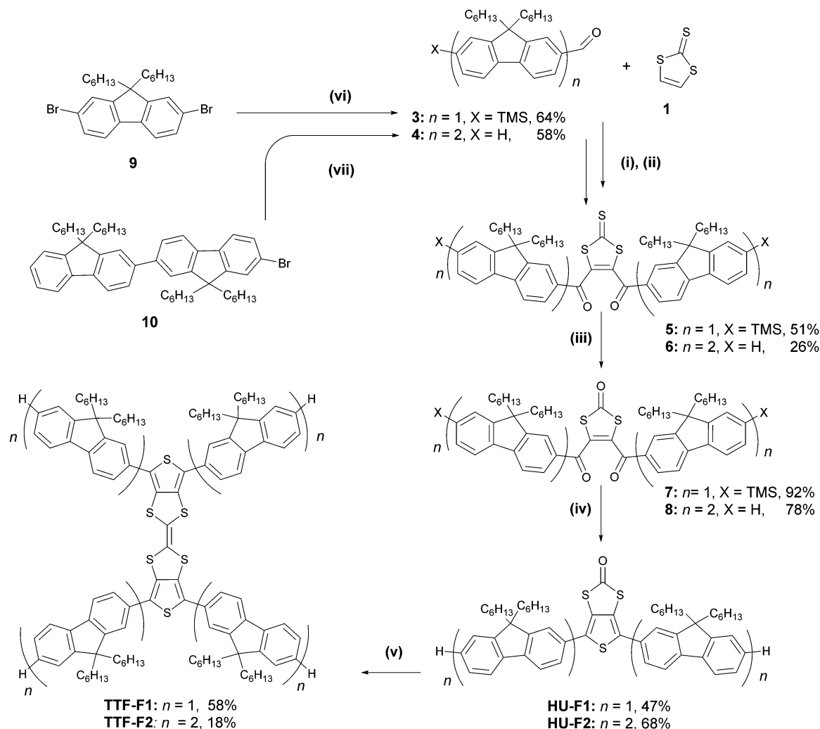
Scheme 1 Synthesis of TTF-Fn ( n = 1, 2 ) through a 1,3-dithiole-2-one core. Reagents and conditions : (i) LDA·THF, THF, -55\text{ }^{\circ}\text{C} ; (ii) \text{MnO}_2 , \text{CH}_2\text{Cl}_2 , rt, 1 min; (iii) \text{Hg}(\text{OAc})_2 , \text{CH}_2\text{Cl}_2/\text{CH}_3\text{COOH} (3 : 1 v/v), rt, overnight; (iv) \text{P}_2\text{S}_5 , \text{NaHCO}_3 , 1,4-dioxane, 90\text{ }^{\circ}\text{C} , 3 h; (v) \text{P}(\text{OEt})_3 , 125\text{ }^{\circ}\text{C} , 3 days; (vi) n\text{-BuLi} , \text{TMSCl} , n\text{-BuLi} , DMF, THF, -78\text{ }^{\circ}\text{C} , overnight; (vii) n\text{-BuLi} , DMF, THF, -78\text{ }^{\circ}\text{C} , overnight.
