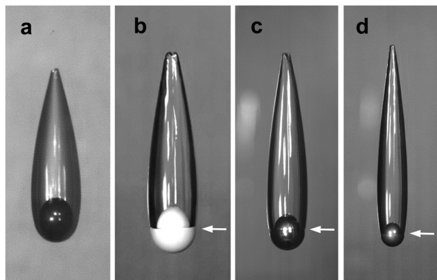
Fig. 1 High-speed camera snapshots of sphere-in-cavity formation for a 10 mm Leidenfrost steel sphere, T_S = 250\text{ }^\circ\text{C} , free falling in PP1 13 (a) and for spheres with attached streamlined air-cavity formation free falling in water using a: (b) 20 mm zirconia sphere; (c) 15 mm steel sphere; and (d) 10 mm tungsten carbide sphere. All spheres in (b–d) have a water contact angle of about 90^\circ and were released from about 2.0 m above the water surface. The cavity–sphere contact line is marked with a white arrow in each image. See Video 1 (ESI † ) for the steady fall of 10 mm zirconia, 10 mm steel and 10 mm tungsten carbide spheres with attached cavities.
