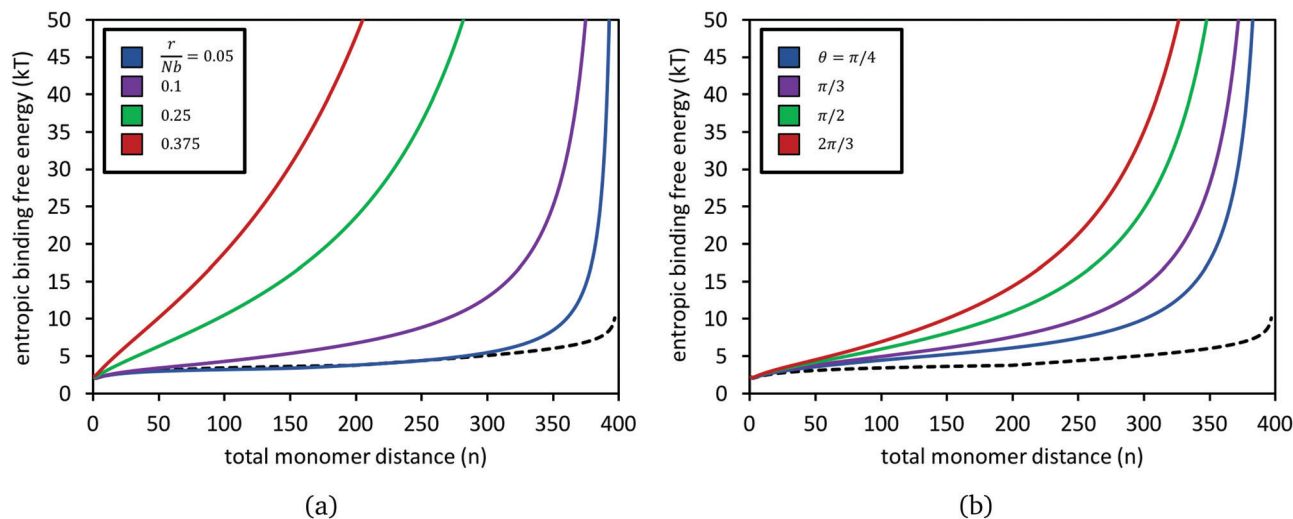
Fig. 4 Entropic binding free energy, \beta\Delta G_{poly}(n;N,r,\theta) , for forming a reversible crosslink at position n_1 + n_2 = n along two polymers of N = 200 segments each, for different choices of chain stretch r at constant angle \theta (panel a), and for different \theta at constant stretch r (panel b). In (a), the two chains are at an angle of \theta = \pi/2 . In (b), the stretch ratio is set to r/Nb = 0.15 . In both panels, the black dashed curve is for when the two polymers have their ends untethered, i.e. eqn (5).
