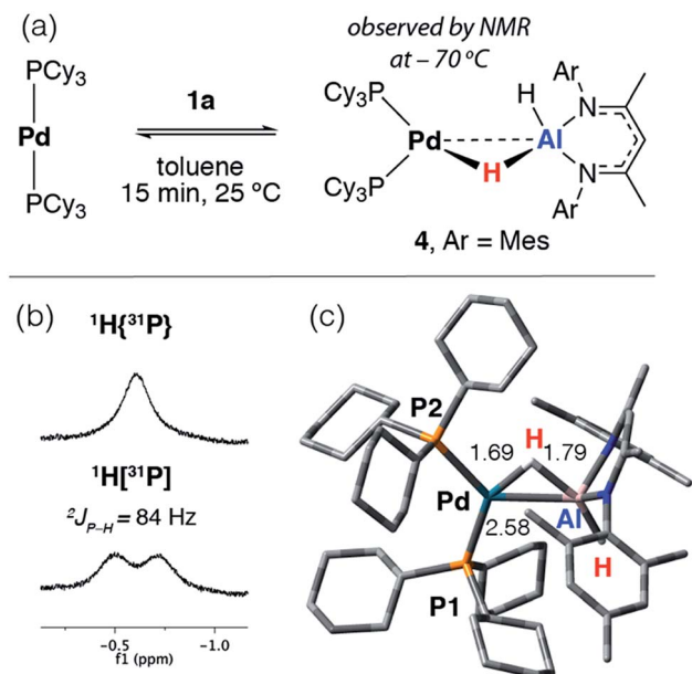
Scheme 2 (a) Reversible reaction of 1a with [\text{Pd}(\text{PCy}_3)_2] . (b) Hydride region of the ^1\text{H}\{^{31}\text{P}\} NMR spectrum at -70 °C in toluene-d 8 . (c) Calculated structure of 4 with selected bond lengths in Å.
