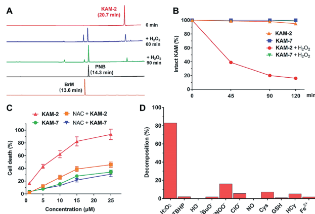
Fig. 2 H 2 O 2 -responsive behaviours of KAM-2 . (A) Decomposition of 100 \mu M KAM-2 in presence of H 2 O 2 (2 eq.) as monitored by RP-HPLC (254 nm). (B) Decomposition of KAM-2 and KAM-7 (100 \mu M) with or without H 2 O 2 (10 eq.). (C) The effects of NAC on the cytotoxicity of KAM-2 and KAM-7 in HL-60 cells after 72 h incubation. (D) Selectivity of KAM-2 toward H 2 O 2 as determined by measuring its decomposition ratios under various stimuli.
