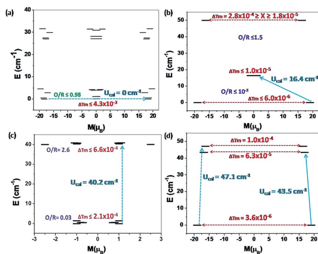
Fig. 10 The ab initio POLY_ANISO computed magnetisation blocking barrier for complexes (a) 1 {Cr 2 Dy 2 }, (b) 3 {Mn 2 Dy 2 }, (c) 5 {Fe 2 Dy 2 } and (d) 7 {Al 2 Dy 2 }. The x-axis indicates the magnetic moment of each state along main magnetic axis of Dy ions, while y-axis denotes the energy of the respective states. The thick black line indicates the Kramer's doublets as a function of computed magnetic moment. The indigo colour shows the possible pathway via Orbach/Raman relaxation. The dotted red lines represent the presence of QTM/TA-QTM between the connecting pairs. The numbers provided are the mean absolute value for the corresponding matrix element of transition magnetic moment. A thick cyan coloured arrow shows the zero field relaxation whereas a dotted cyan coloured arrow shows relaxation in an applied external field.
