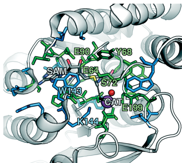
Fig. 1 COMT structure with SAM and CAT substrates shown in gray along with Mg^{2+} as a magenta sphere and a water coordinating the Mg^{2+} as a red sphere. The 28 protein residues (518 atoms with H atoms) included in a large QM region, as described in the main text, are shown as sticks. A subset that was identified by systematic analysis of QM regions is shown in green, whereas the remainder is shown in blue. Specific residues of interest are labeled by their single letter residue code and number.
