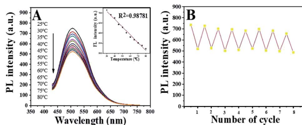
Fig. 5 (A) PL spectra of N-CDs obtained in the temperature range of 25\text{--}80\text{ }^\circ\text{C} (inset: the emission intensity as a function of temperature). (B) Reversible fluorescence response of eight consecutive cycles from 25\text{ }^\circ\text{C} to 80\text{ }^\circ\text{C} .
