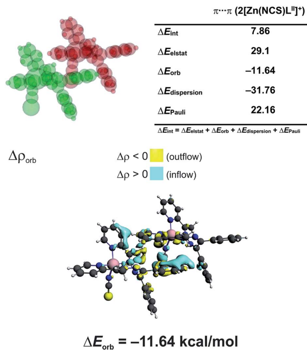
Fig. 6 (top) ETS-NOCV outcomes scrutinizing the nature of ionic interaction between two \pi -stacked [Zn(NCS)L]^+ units in 3 . (bottom) The overall change in electron density \Delta \rho_{\text{orb}} with the corresponding energy \Delta E_{\text{orb}} .
