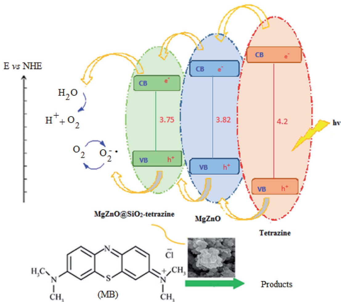
Scheme 1 Proposed photocatalysis mechanism for MgZnO@SiO 2 -tetrazine.
