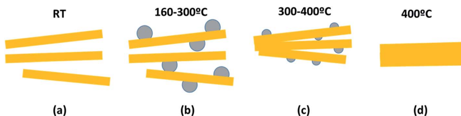
Scheme 1 Thermally-induced silver migration in \beta - \text{AgVO}_3 nanoribbons.
