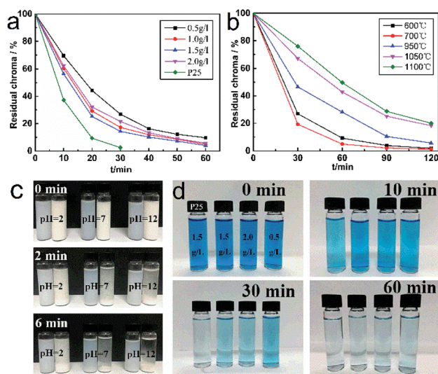
Fig. 9 (a) Photocatalytic activity of \text{TiO}_2 whiskers calcined at 700 °C with different addition amounts. (b) Photocatalytic activity of \text{TiO}_2 whiskers calcined at different temperatures. (c) Settlement properties of whiskers in aqueous solutions at different pH values. (d) Digital photographs of the photocatalytic decolorization of MB with different addition amounts.
