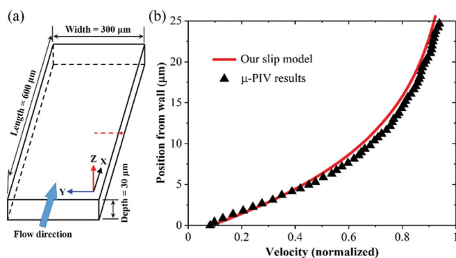
Fig. 4 (a) Geometry of the microchannel for slip model validation. (b) Velocity profiles from experiment and simulation along the line of x = 300 μm and z = 15 μm; the x-axis is the velocity normalized by the free stream velocity and the y-axis is the distance from the wall.
