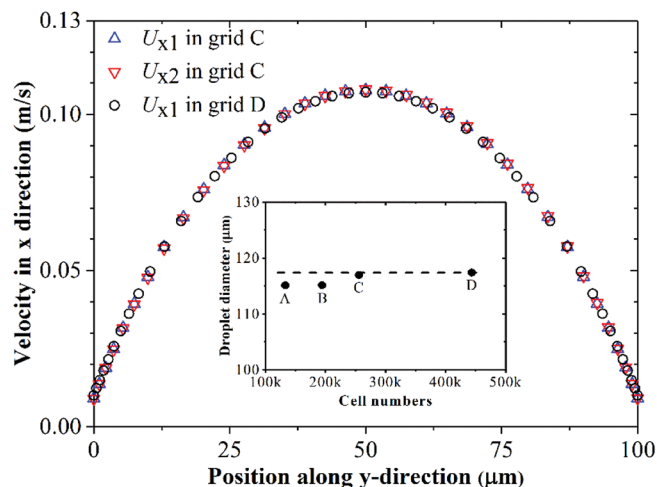
Fig. 3 Grid independence study for Q_d = 0.2 mL h -1 and Q_c = 2 mL h -1 with moderate slip lengths of 2 μm. U_{x1} and U_{x2} represent the x-velocity along the y-direction at x = 100 μm and x = 150 μm on the symmetry plane, respectively.
