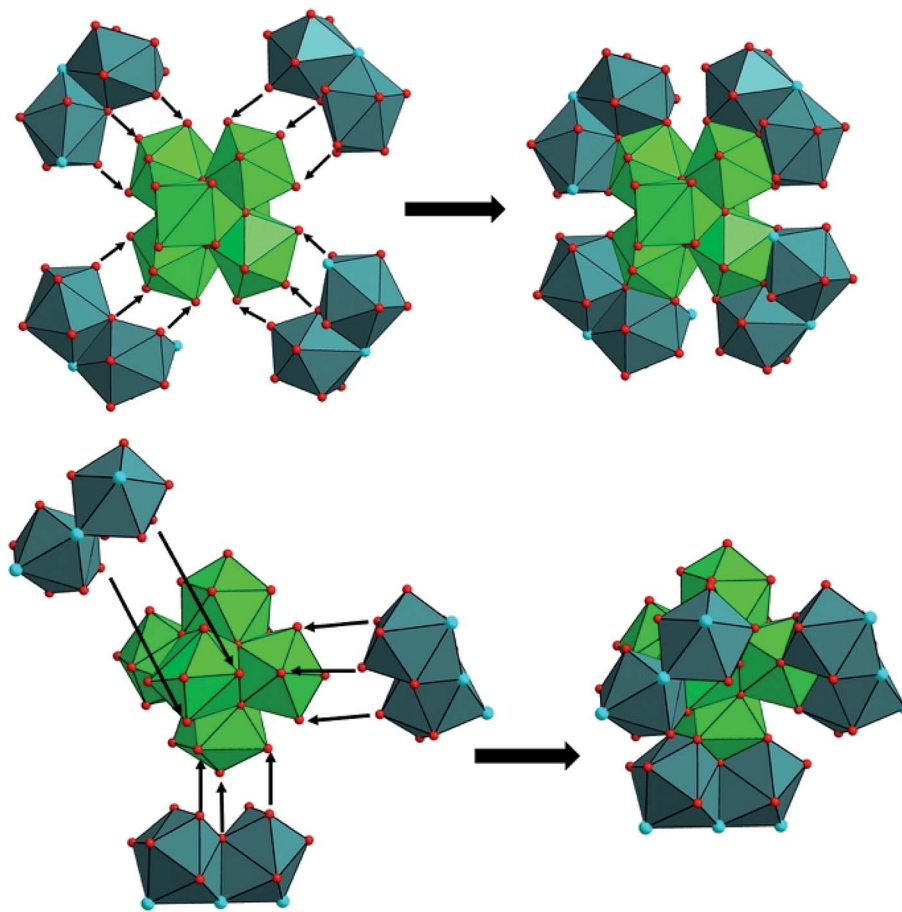
Fig. 7 Different connection manners between the central hexanuclear core [\text{U}_6\text{O}_4(\text{OH})_4] and peripheral dinuclear uranium sub-units to form different uranium clusters (top; \{\text{U}_{14}\} , bottom; \{\text{U}_{12}\} ). 39
