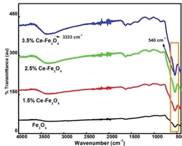
Fig. 2 FTIR spectra of pure \text{Fe}_3\text{O}_4 and doped \text{Fe}_3\text{O}_4 .
