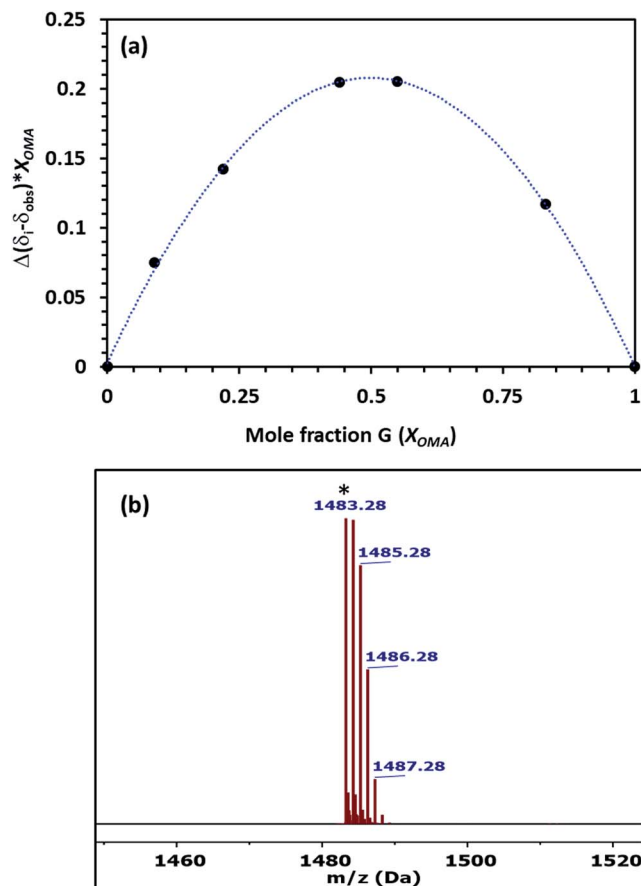
Fig. 3 (a) Job's plot of Pillar-1 with OMA determined from ^1\text{H} NMR titration in \text{CDCl}_3 at 25^\circ\text{C} . (b) ES-MS spectrum of [(\text{Pillar-1} \supset \text{OMA})\text{-PF}_6]^+ .
