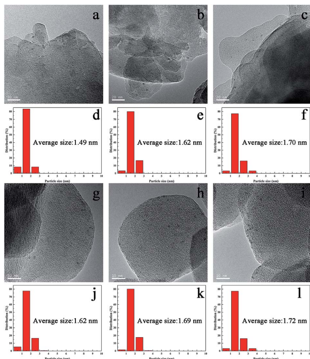
Fig. 3 HRTEM images and metal particle size distributions of the Pd@TS-1 and Pd@HTS-1 before and after high-temperature oxidation–reduction–oxidation treatments. (a, d) Pd@TS-1-O. (b, e) Pd@TS-1-OR. (c, f) Pd@TS-1-ORO. (g, j) Pd@HTS-1-O. (h, k) Pd@HTS-1-OR. (i, l) Pd@HTS-1-ORO.)
