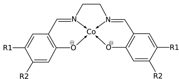
Fig. 2 Structure of Co(salen) ( R_1 = R_2 = \text{H} ), salen = N,N' -bis(salicylaldehyde)-ethylenediimino ligand. R_1 and R_2 are sites for substitution.
