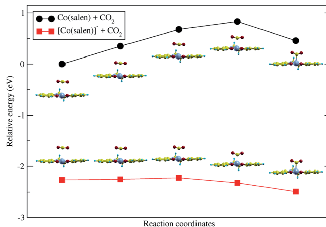
Fig. 3 Nudged elastic band calculation shows that the formation of (top) neutral Co(salen)- \text{CO}_2 complex is unfavored. The forward activation energy for this reaction is 0.828 eV. The formation of (bottom) [\text{Co}(\text{salen})\text{-CO}_2]^- is favored with a forward activation energy of 0.042 eV.
