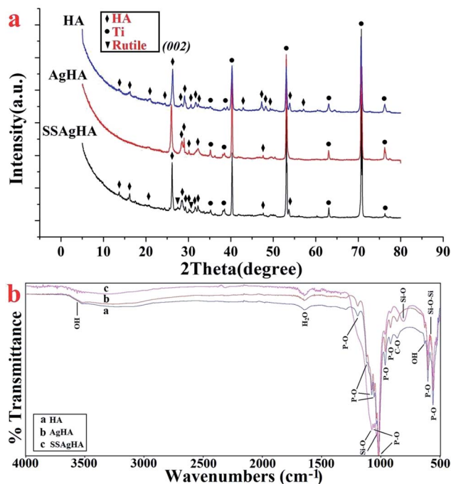
Fig. 3 XRD pattern (a) and FT-IR spectra (b) of the HA, AgHA and SSagHA/Ti coatings that were deposited on their underlying Ti substrates.
