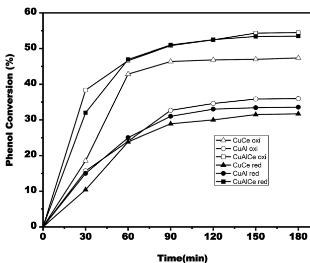
Fig. 13 Evolution of phenol conversion during single run catalytic tests for CuCe oxi ( \Delta ), CuCe red ( \blacktriangle ), CuAl oxi ( \circ ), CuAl red ( \bullet ), CuAlCe oxi ( \square ), CuAlCe red ( \blacksquare ).
