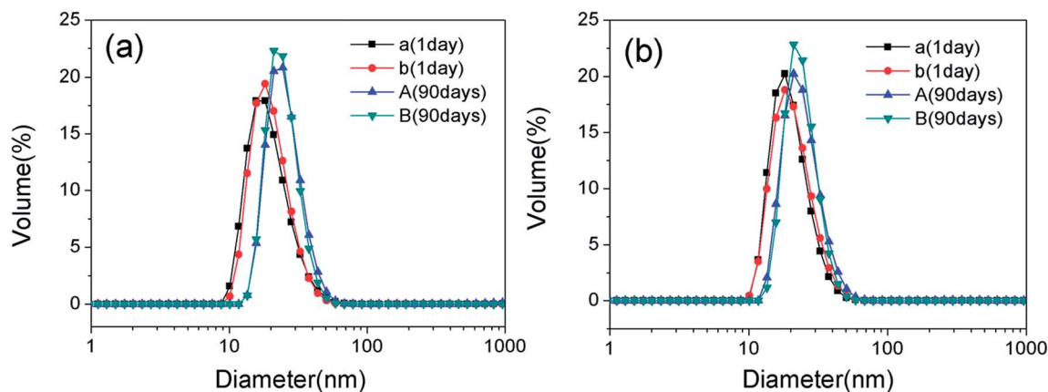
Fig. 7 Nanoemulsion droplet sizes measured by DLS. (a) Size variation of the nanoemulsions with 0.15% w/v G16-2-16 stored for 1 day and 90 days ((a) and A) without OMT; (b) size variation of the nanoemulsions with 0.20% w/v G16-2-16 stored for 1 day and 90 days ((a) and A) without OMT; (b) size variation of the nanoemulsions with 0.20% w/v G16-2-16 stored for 1 day and 90 days ((b) and B) with 3.4 \times 10^{-3}\% w/v OMT).
