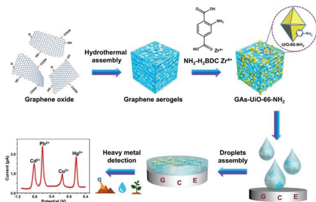
Fig. 7 Synthesis of the GAs-Uio-66- \text{NH}_2 composite via the in situ growth of the Uio-66- \text{NH}_2 crystal on the GAs Matrix and the determination of heavy metal ions with the modified electrode. Reprinted from ref. 74 with permission from American Chemical Society.
