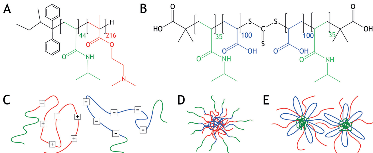
Fig. 1 Chemical structures of (a) cationic PNIPAM- b -PDMAAEMA, which was synthesized by anionic polymerization, and (b) PNIPAM- b -PAA- b -PNIPAM, which was synthesized by reversible addition fragmentation chain transfer (RAFT) polymerization. Schematic representations of (c) PNIPAM- b -PDMAAEMA and PNIPAM- b -PAA- b -PNIPAM, (d) a C3M, and (e) PCMs. The red block represents PDMAAEMA, the blue block PAA and the green blocks PNIPAM.
