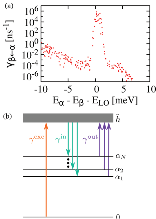
Fig. 1 (a) Calculated phonon scattering rate \gamma_{\beta \leftarrow \alpha} of the 21 \times 7 \text{ nm}^2 platelet as a function of the energy difference E_\alpha - E_\beta of the involved initial ( \alpha ) and final states ( \beta ). The energy difference is plotted as detuning from the mean LO phonon energy E_{\text{LO}} = \hbar(\omega_{\text{LO}}^i + \omega_{\text{LO}}^f)/2 . The increasing background is given by acoustic phonon scattering, which peaks zero absolute energy ( -25.5 \text{ meV} in this relative scale). (b) Schematic of the Lindblad processes involving the high-energy band \tilde{h} .
