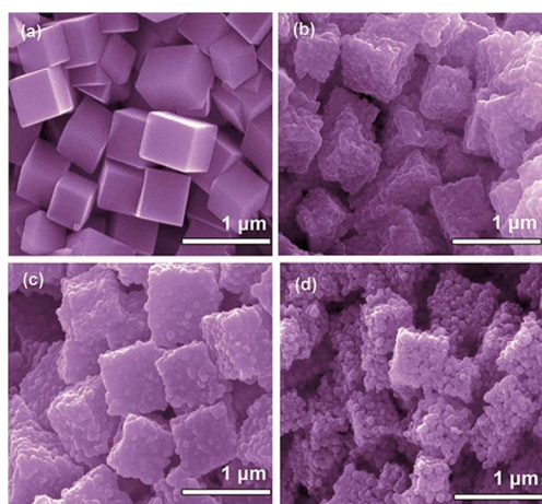
Fig. 15 SEM images of the as-prepared PB nanocubes (a) and \text{Fe}/\text{C} nanocubes obtained at different pyrolysis temperatures: (b) 600 °C, (c) 650 °C and (d) 700 °C 150 – reproduced by permission of the Royal Society of Chemistry.
