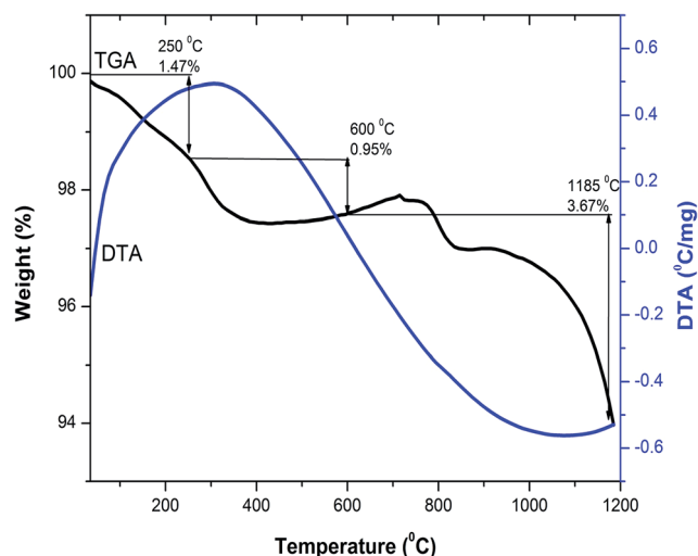
Fig. 1 Combined differential thermal analysis (DTA) and thermogravimetric analysis (TGA) curves of \text{Y}_2\text{Ce}_1\text{Fe}_5\text{O}_{12} composition.
